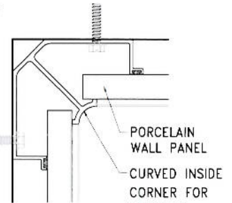
Inside Corner
