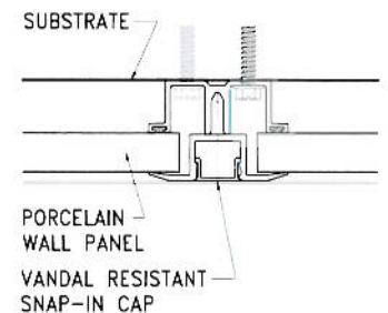
Vertical Mullion
