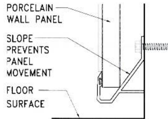
Sill
