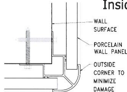
Outside Corner
